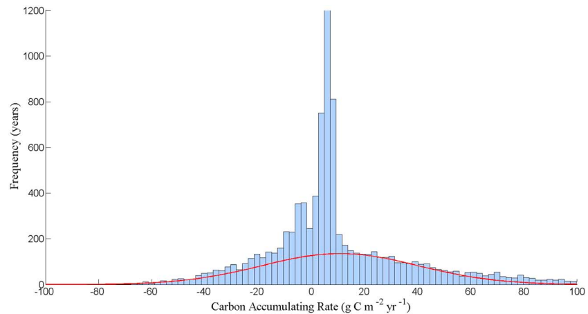
Figure 6. Frequency histogram of simulated peat carbon accumulation rates from 15 ka to 5 ka, characterized with a normal distribution ( \mu = 10.82 \text{ g C m}^{-2} \text{ yr}^{-1} and \sigma = 29.22 \text{ g C m}^{-2} \text{ yr}^{-1} ).
