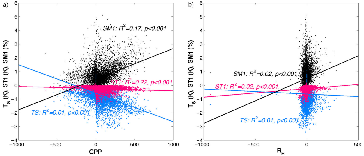
Fig. 11. Scatterplots of aerosol-induced changes of key carbon fluxes (GPP and R_H ) and environmental conditions ( T_s , ST1 and SM1). Units for the carbon fluxes are g C m^{-2} yr^{-1} .
