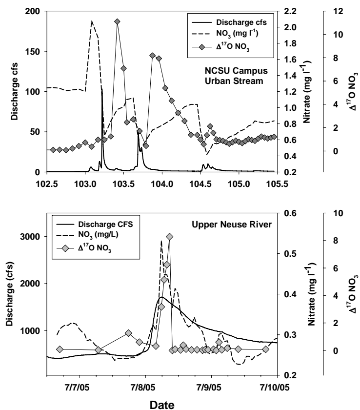
Figure 4. \Delta^{17}\text{O NO}_3 , discharge and nitrate concentrations in a small urban stream and the upper river near Raleigh NC. The \Delta^{17}\text{O} on the right axis can be converted to \text{NO}_3^-_{\text{atm}} by dividing by 21‰, this regions deposition value. If the assumption of a homogenous nitrate pool that is incorporated into hydrologic models were true, we should see no change in isotopes with changing source strength. This is clearly not observed. The \Delta^{17}\text{O} peak values do not correspond to the peak nitrate concentrations or the discharge peaks, but occur during falling portions of the hydrographs. This behavior is due changes of export probability of \text{NO}_3^-_{\text{atm}} that accumulated on the surface during the dry season, which is being flushed past the plant and bacterial biomass by the rain. The upper Neuse River exhibits different behavior with \text{NO}_3^-_{\text{atm}} more closely aligned with discharge and concentration changes. This highlights then nitrate source flux differences for biogeochemically different systems.
