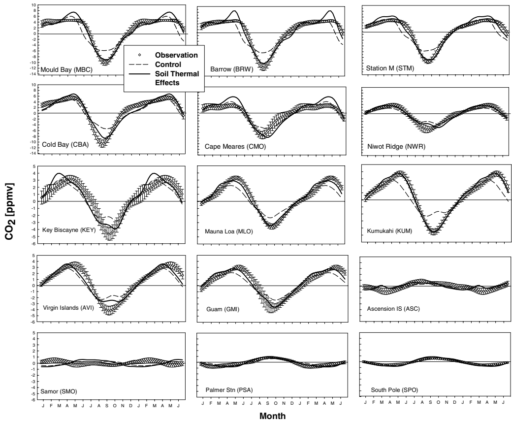
Fig. 4. Comparisons between the observed seasonal cycle of CO 2 and simulated seasonal cycle for 15 monitoring stations of the NOAA/CMDL network. The mean and standard deviation from 1982 to 1995 are shown for the observed data. The simulated CO 2 concentrations were estimated by providing the monthly NCE estimates of the TEM 5.0 simulation (soil thermal effects, solid line) and the TEM 4.2 simulation (control, dashed line) to the Model of Atmosphere and Transport Chemistry (MATCH). The first 6 months of each cycle are displayed twice to reveal the annual variation more clearly.
