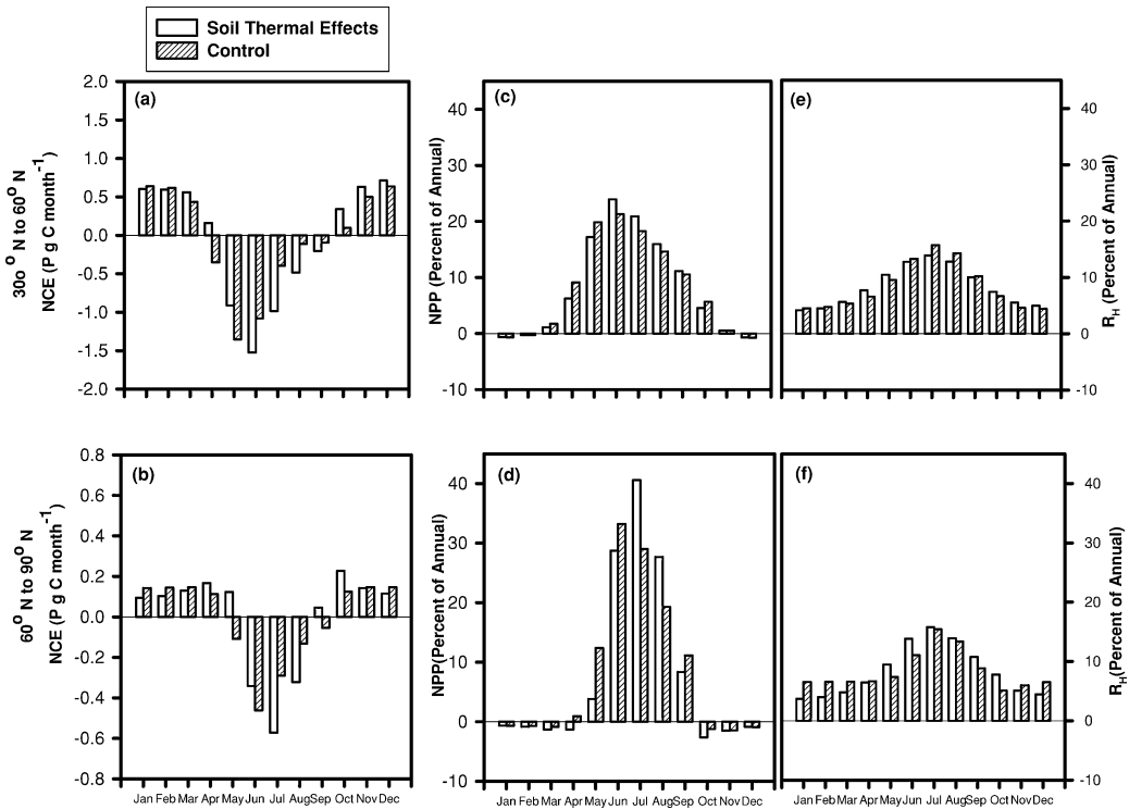
Fig. 3. Monthly simulated net carbon exchange (NCE, left panels) and heterotrophic respiration ( R_H , right panels) as estimated by TEM 5.0 and its control simulations for 30–60°N (top panels: a, c and e) and 60–90°N (bottom panels: b, d and f). The simulations are from S2 simulations of the two versions of TEM. The TEM 5.0 simulations are indicated with open bars, and control simulations with hatched bars.
